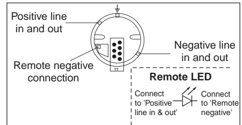
LED Driver Base part no 45681-501
