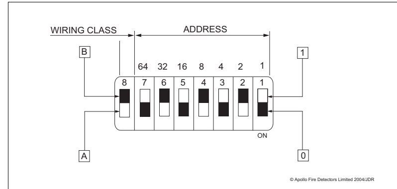
Fig 3. DIL Switch
