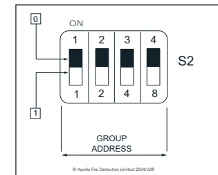
Fig 4. DIP Switch, S2
