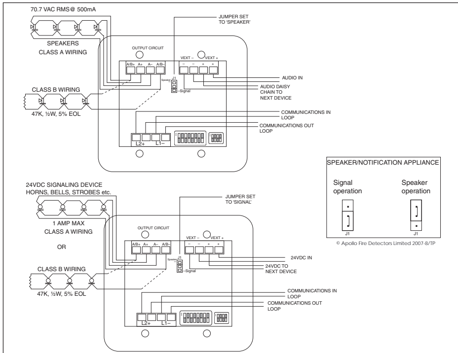
Fig 2. Wiring diagram for XP95A Sounder Control Module
