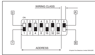
Fig 3. DIP Switch, S1
