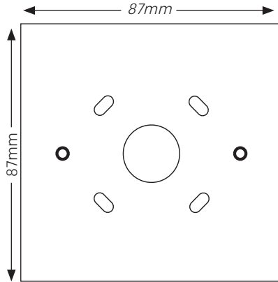
Fig 1 Backbox
