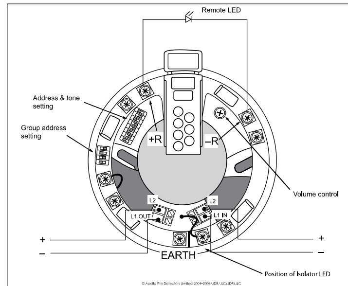
Group Address Settings Fig. 1 Sounder VAD Base with isolator wiring
